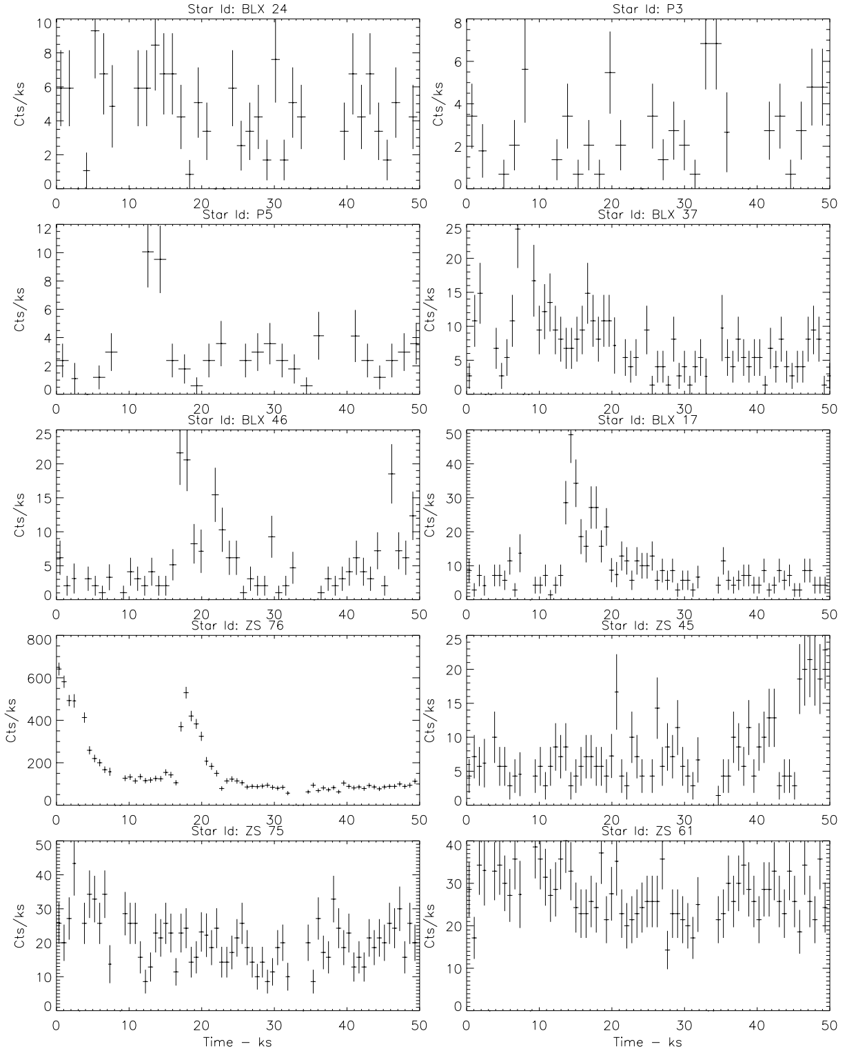
Fig. 1. Light curves of Blanco 1 X-ray variable stars.
